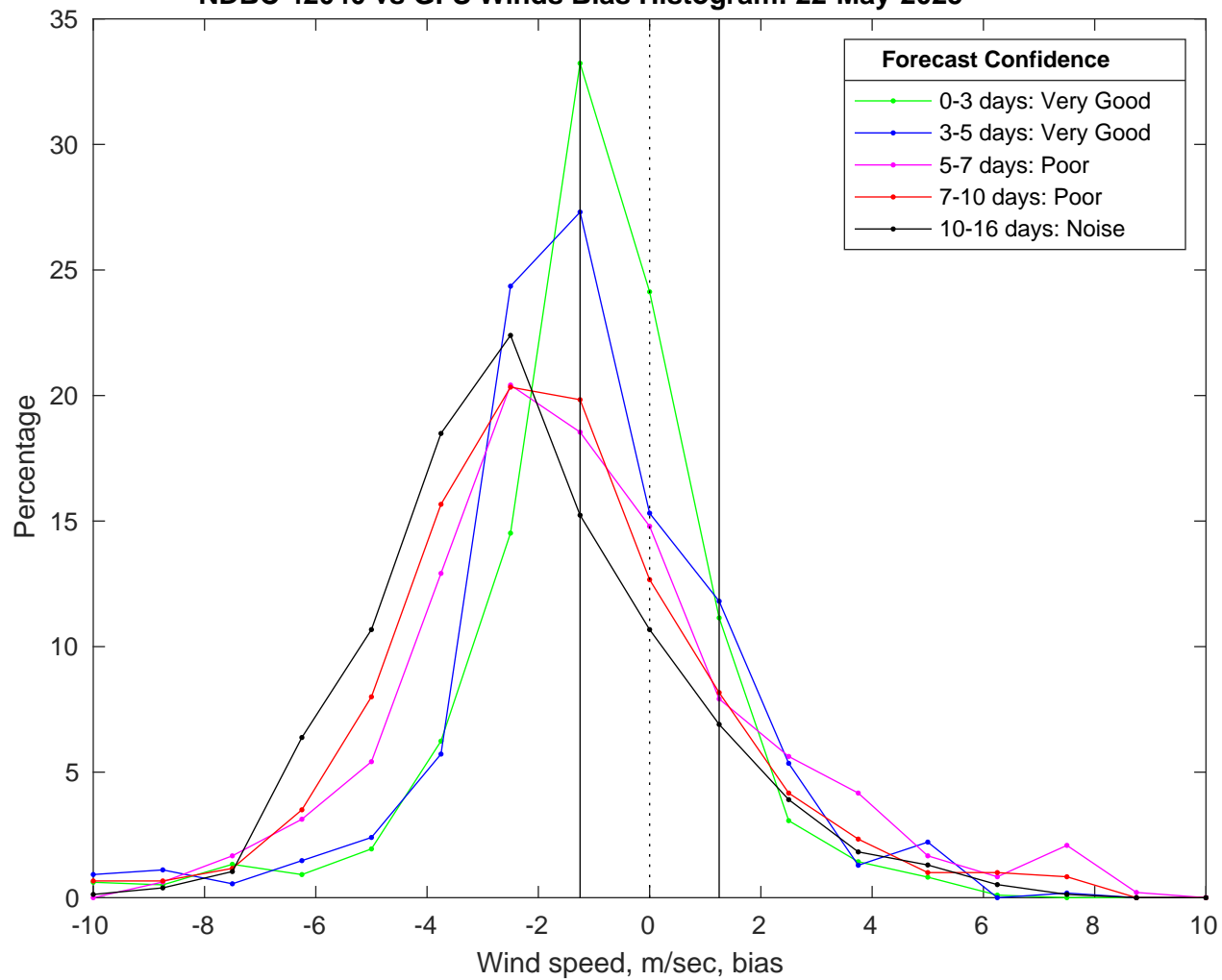
NDBC 42040 vs GFS Winds Bias Histogram: 22-May-2025
