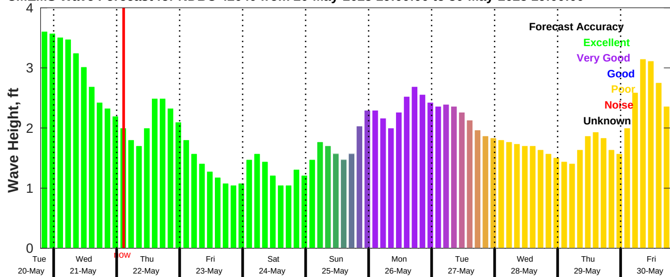
CMEMS Wave Forecast for NDBC 42040 from 20-May-2025 19:00:00 to 30-May-2025 19:00:00
