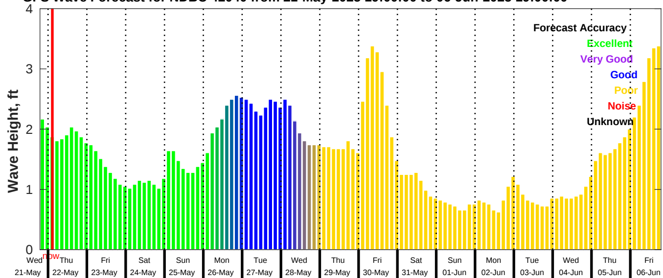
GFS Wave Forecast for NDBC 42040 from 21-May-2025 19:00:00 to 06-Jun-2025 19:00:00
