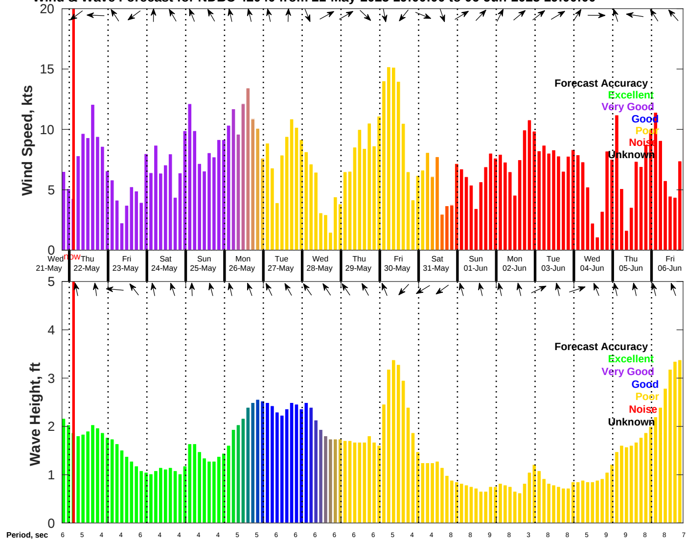
Wind & Wave Forecast for NDBC 42040 from 21-May-2025 19:00:00 to 06-Jun-2025 19:00:00
