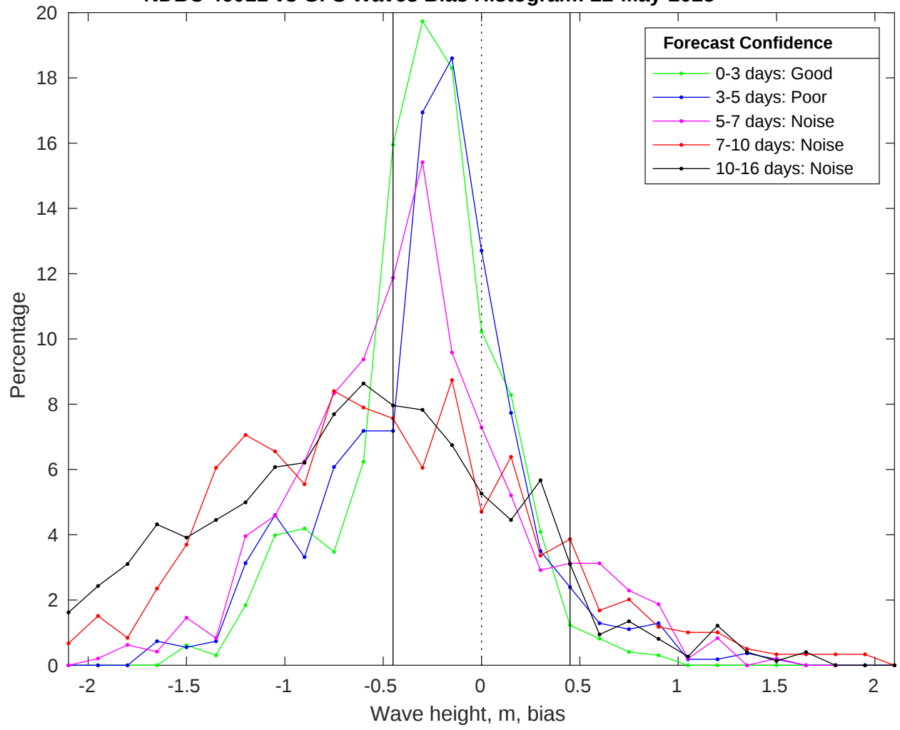
NDBC 46011 vs GFS Waves Bias Histogram: 22-May-2025
