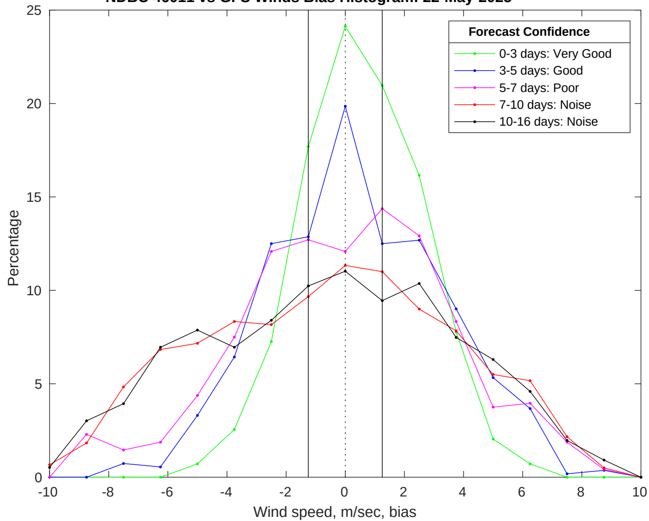
NDBC 46011 vs GFS Winds Bias Histogram: 22-May-2025
