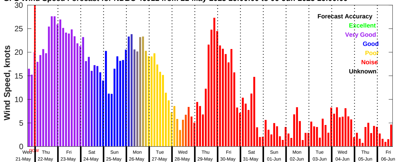
GFS Wind Speed Forecast for NDBC 46011 from 21-May-2025 16:00:00 to 06-Jun-2025 16:00:00
