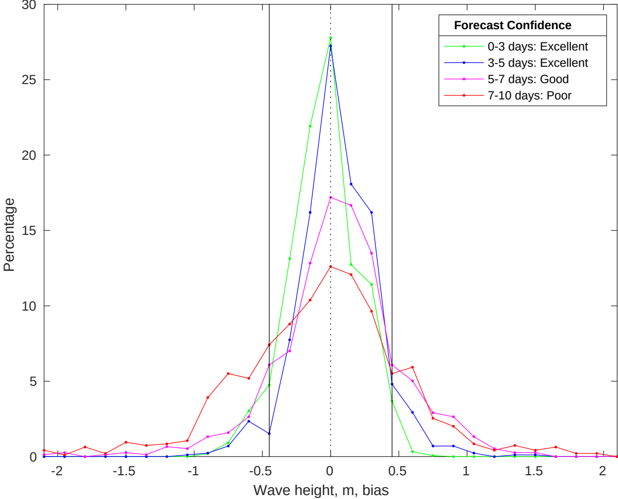
NDBC 46028 vs CMEMS Waves Bias Histogram: 22-May-2025
