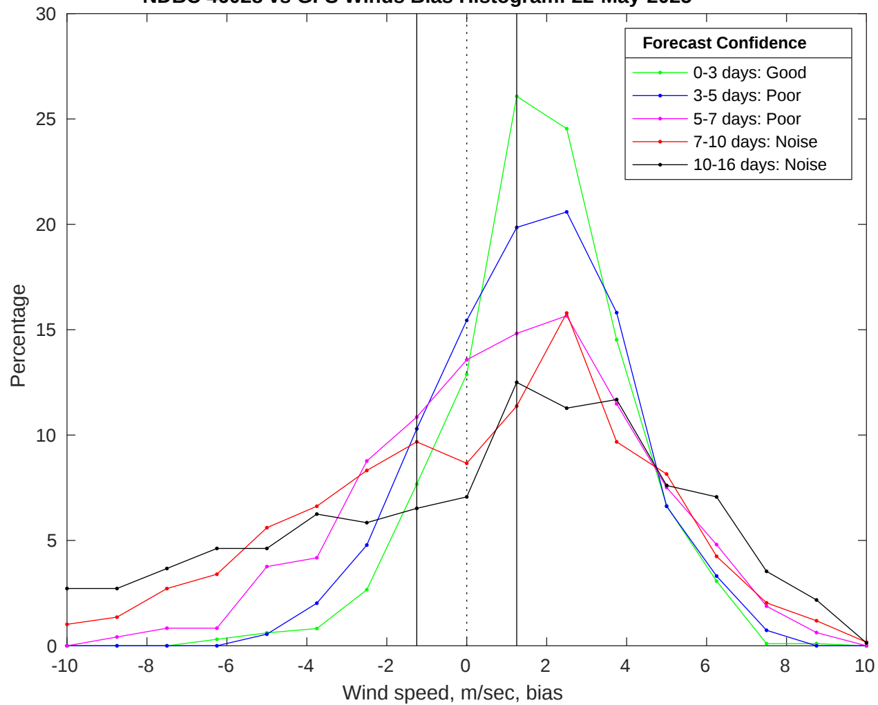
NDBC 46028 vs GFS Winds Bias Histogram: 22-May-2025
