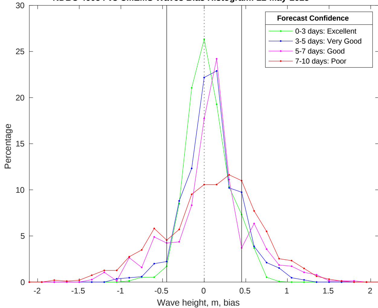
NDBC 46054 vs CMEMS Waves Bias Histogram: 22-May-2025
