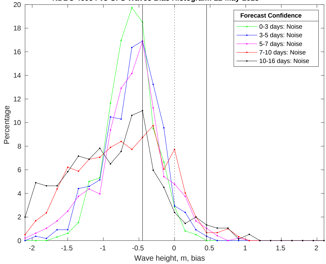
NDBC 46054 vs GFS Waves Bias Histogram: 22-May-2025
