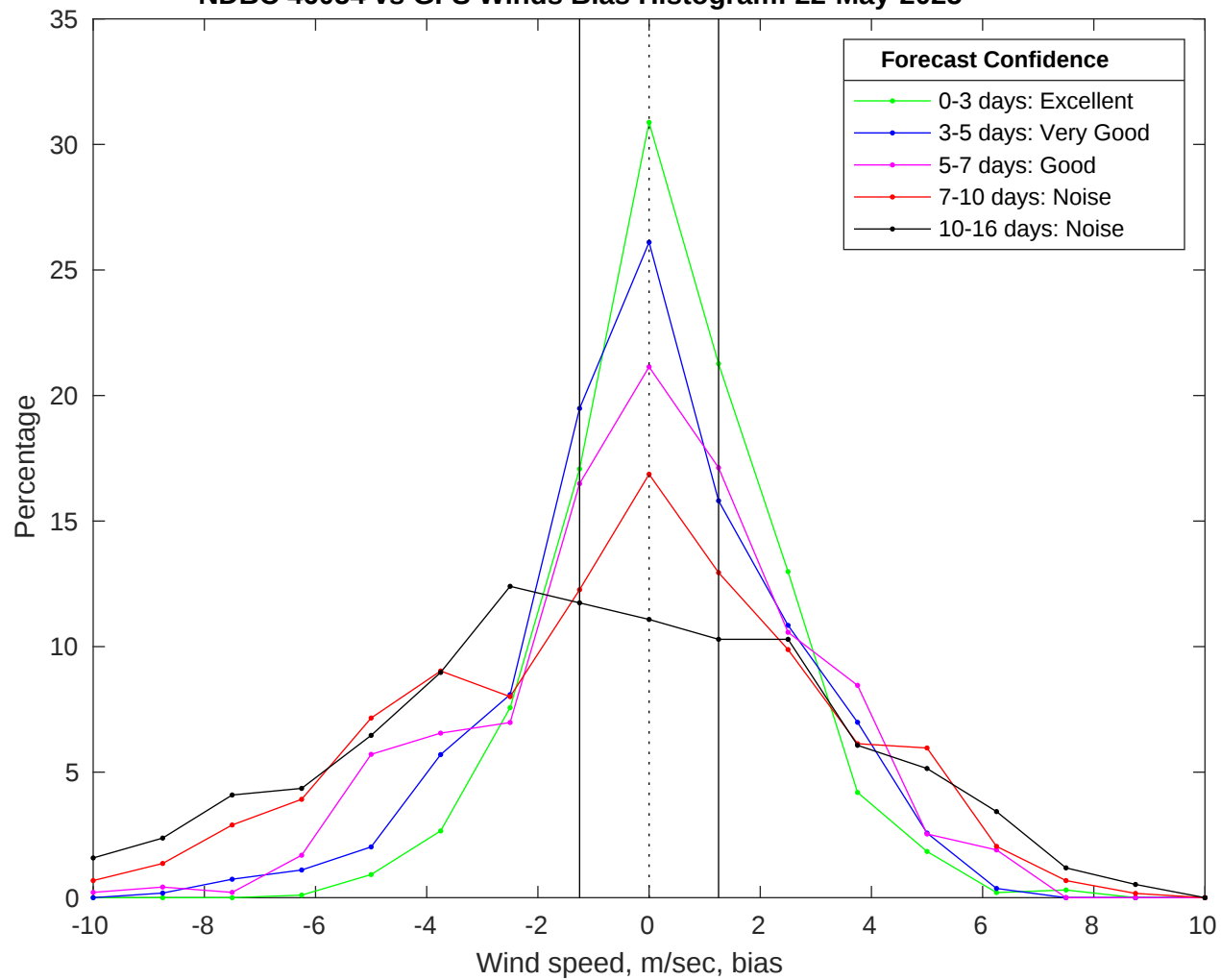
NDBC 46054 vs GFS Winds Bias Histogram: 22-May-2025
