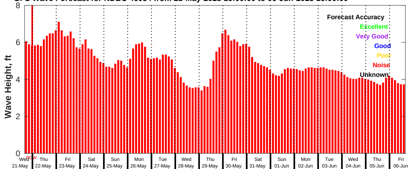
GFS Wave Forecast for NDBC 46054 from 21-May-2025 16:00:00 to 06-Jun-2025 16:00:00
