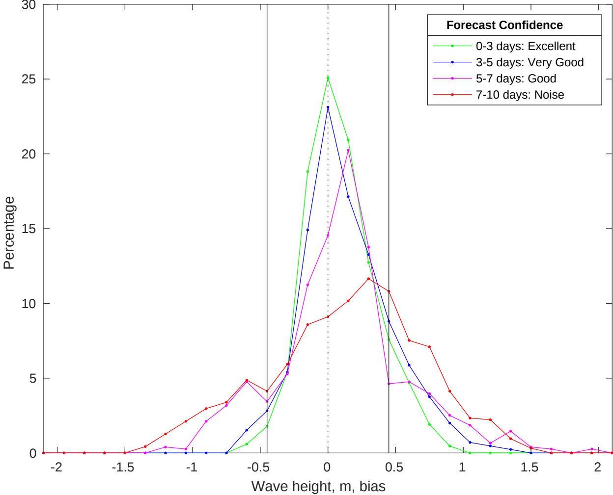
NDBC 46069 vs CMEMS Waves Bias Histogram: 22-May-2025
