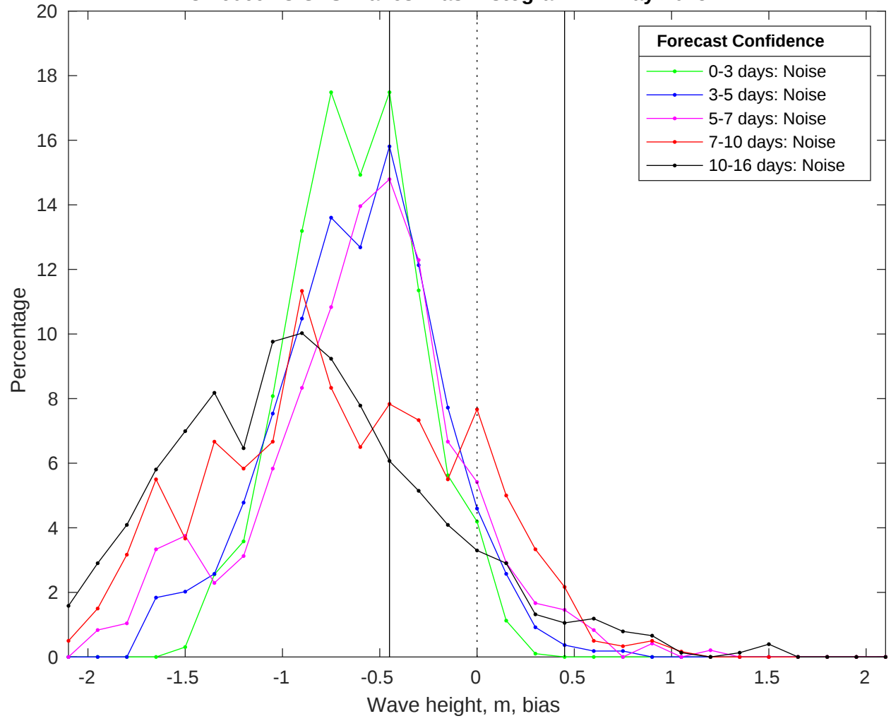
NDBC 46069 vs GFS Waves Bias Histogram: 22-May-2025
