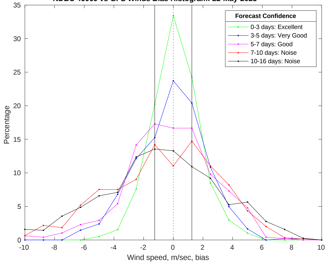
NDBC 46069 vs GFS Winds Bias Histogram: 22-May-2025
