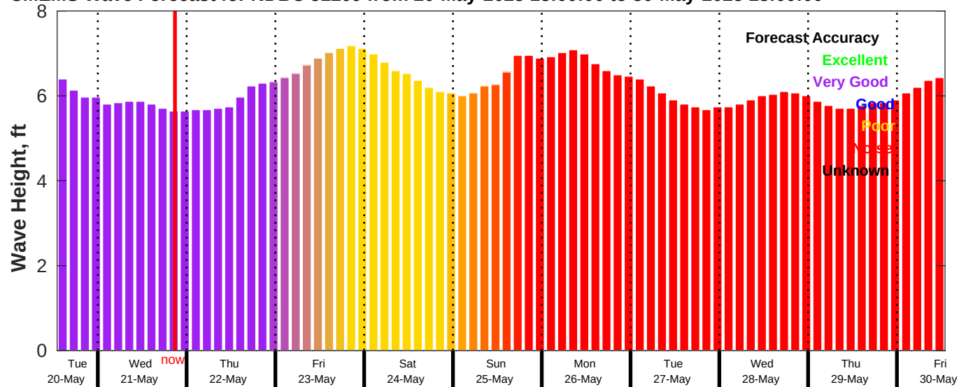
CMEMS Wave Forecast for NDBC 51209 from 20-May-2025 13:00:00 to 30-May-2025 13:00:00
