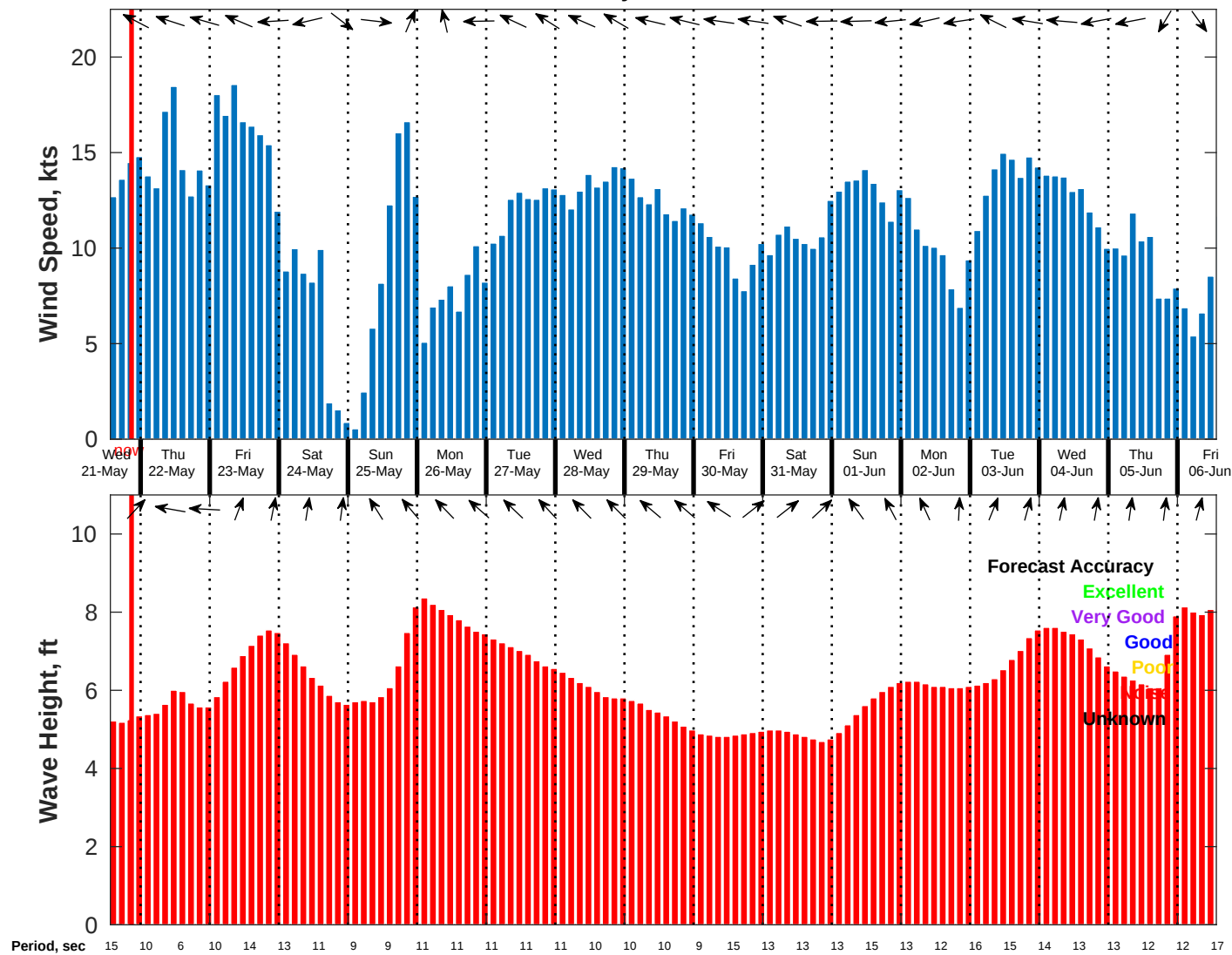
Wind & Wave Forecast for NDBC 51209 from 21-May-2025 13:00:00 to 06-Jun-2025 13:00:00
