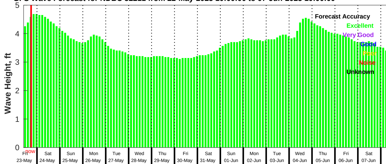
GFS Wave Forecast for NDBC 52211 from 22-May-2025 10:00:00 to 07-Jun-2025 10:00:00
