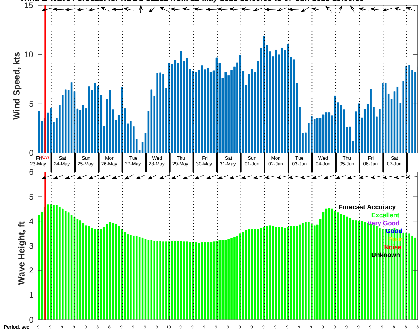
Wind & Wave Forecast for NDBC 52211 from 22-May-2025 10:00:00 to 07-Jun-2025 10:00:00
