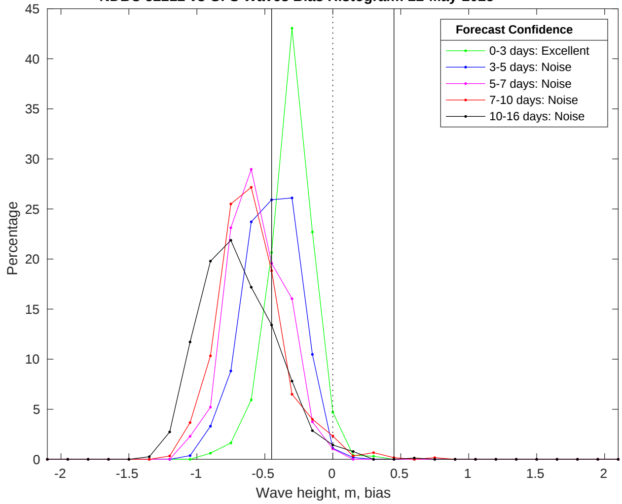
NDBC 52212 vs GFS Waves Bias Histogram: 22-May-2025
