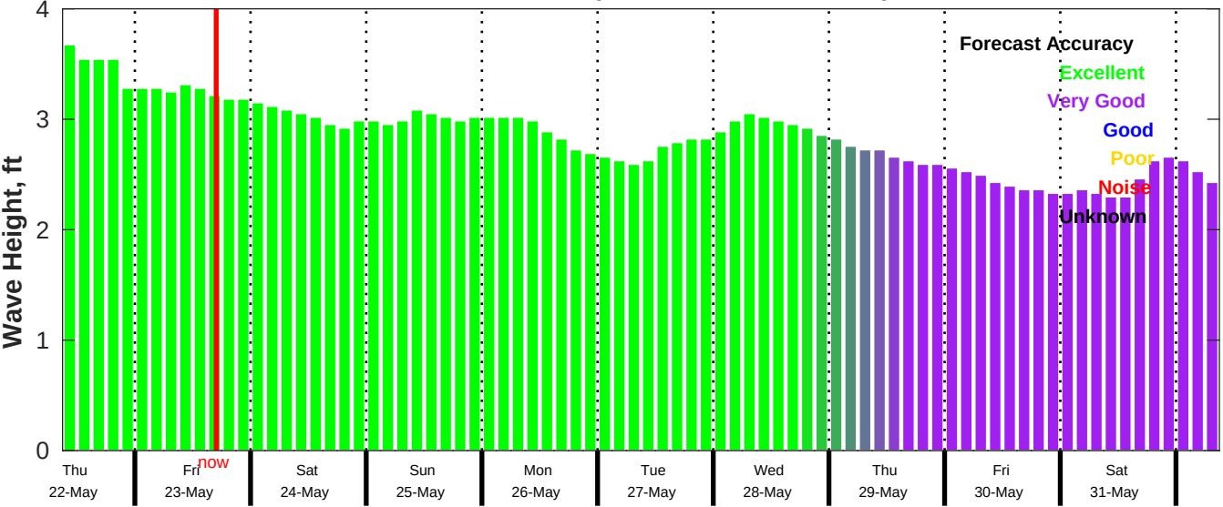
CMEMS Wave Forecast for NDBC 52212 from 21-May-2025 09:00:00 to 31-May-2025 09:00:00
