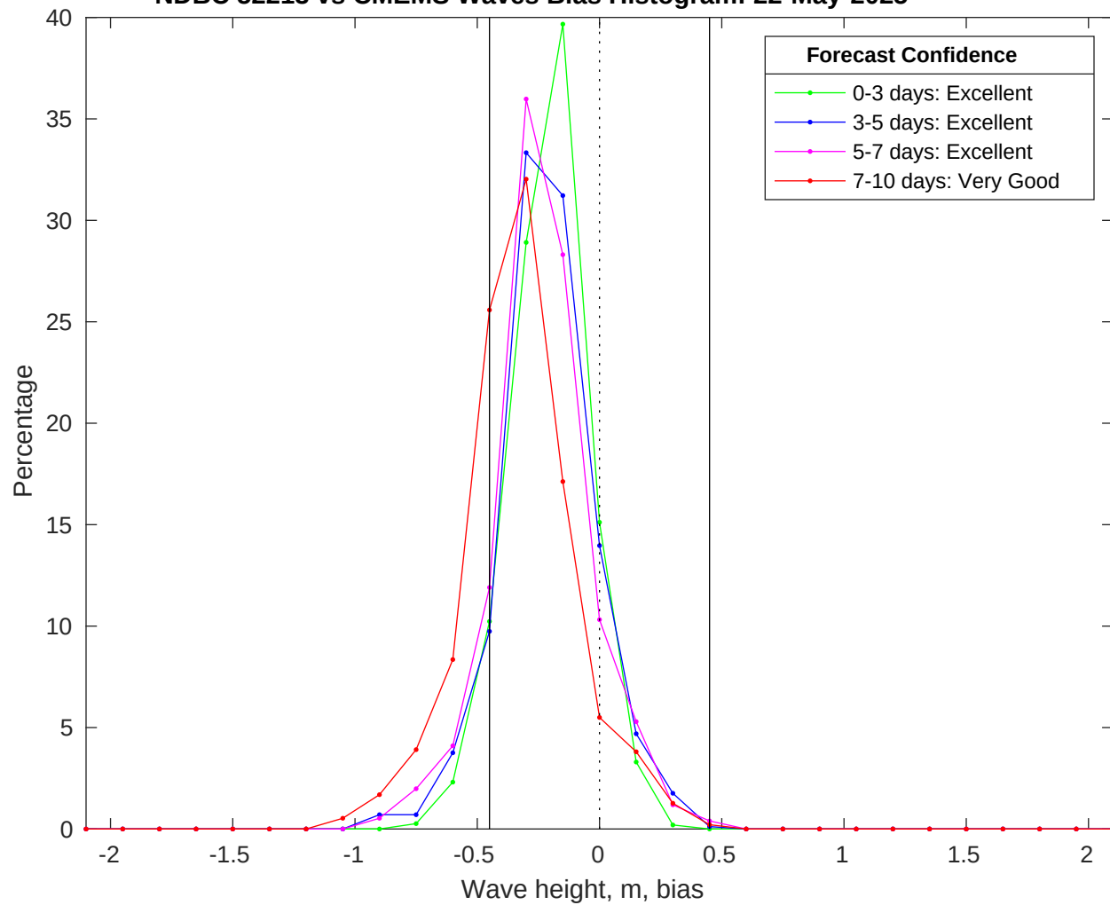
NDBC 52213 vs CMEMS Waves Bias Histogram: 22-May-2025
