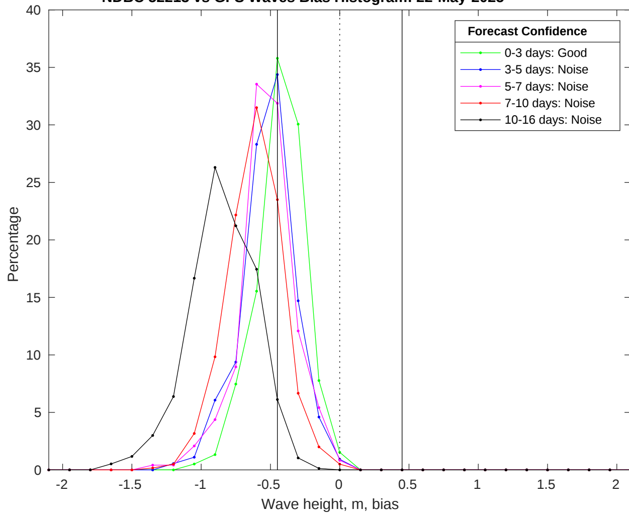
NDBC 52213 vs GFS Waves Bias Histogram: 22-May-2025
