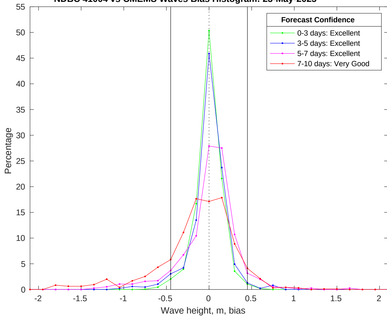
NDBC 41004 vs CMEMS Waves Bias Histogram: 23-May-2025
