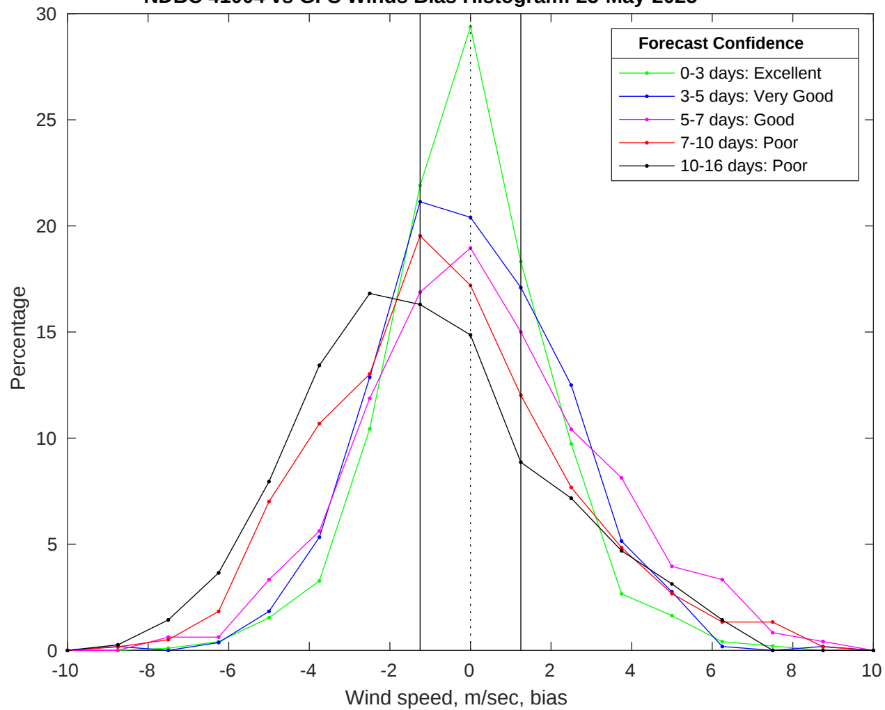
NDBC 41004 vs GFS Winds Bias Histogram: 23-May-2025
