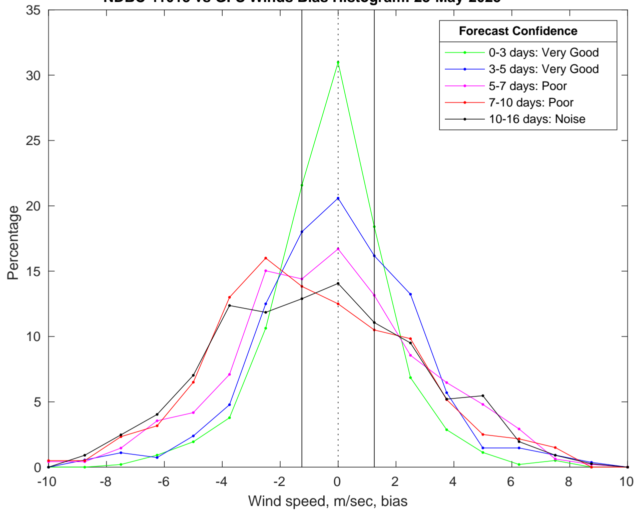
NDBC 41013 vs GFS Winds Bias Histogram: 23-May-2025
