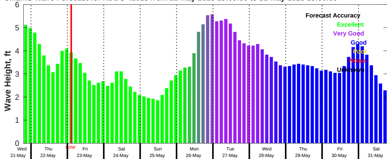
CMEMS Wave Forecast for NDBC 41013 from 21-May-2025 19:00:00 to 31-May-2025 19:00:00
