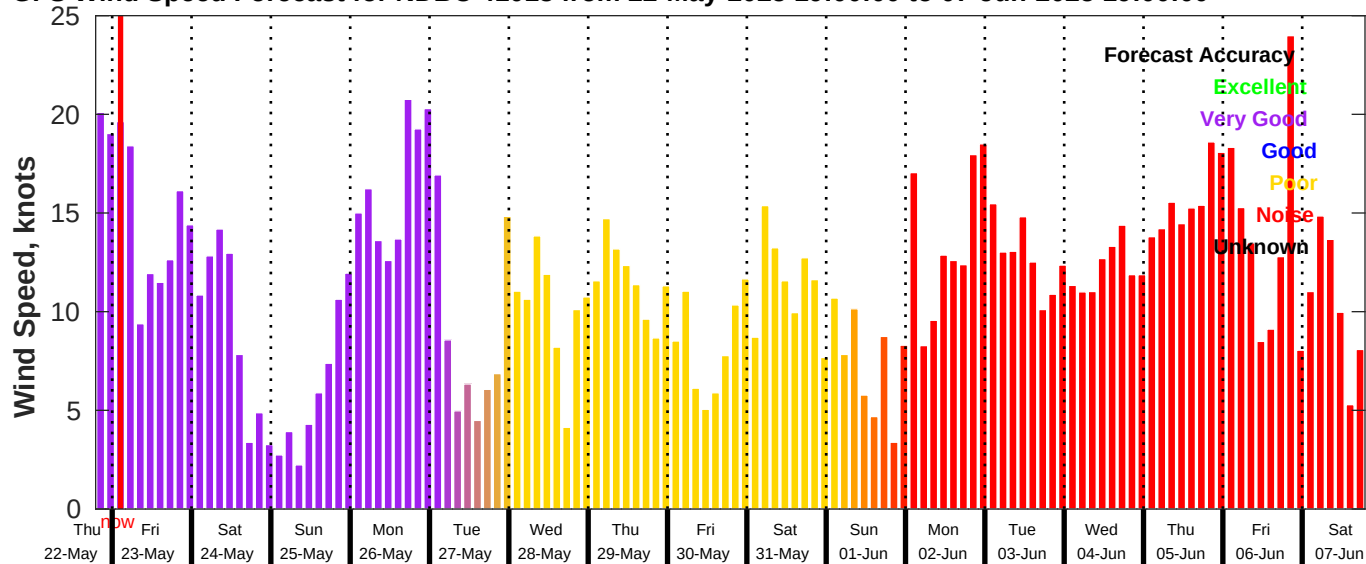
GFS Wind Speed Forecast for NDBC 41013 from 22-May-2025 19:00:00 to 07-Jun-2025 19:00:00
