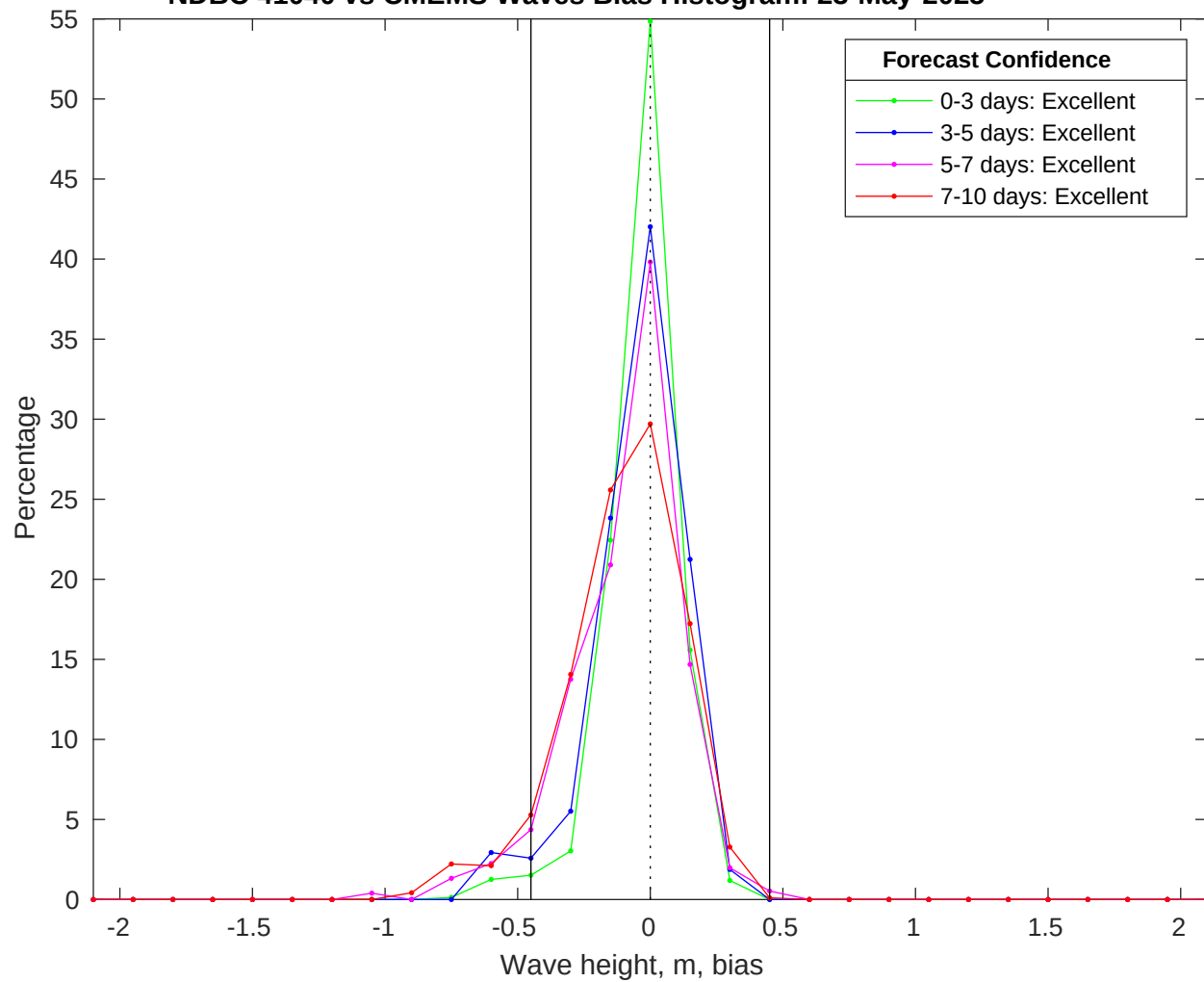
NDBC 41040 vs CMEMS Waves Bias Histogram: 23-May-2025
