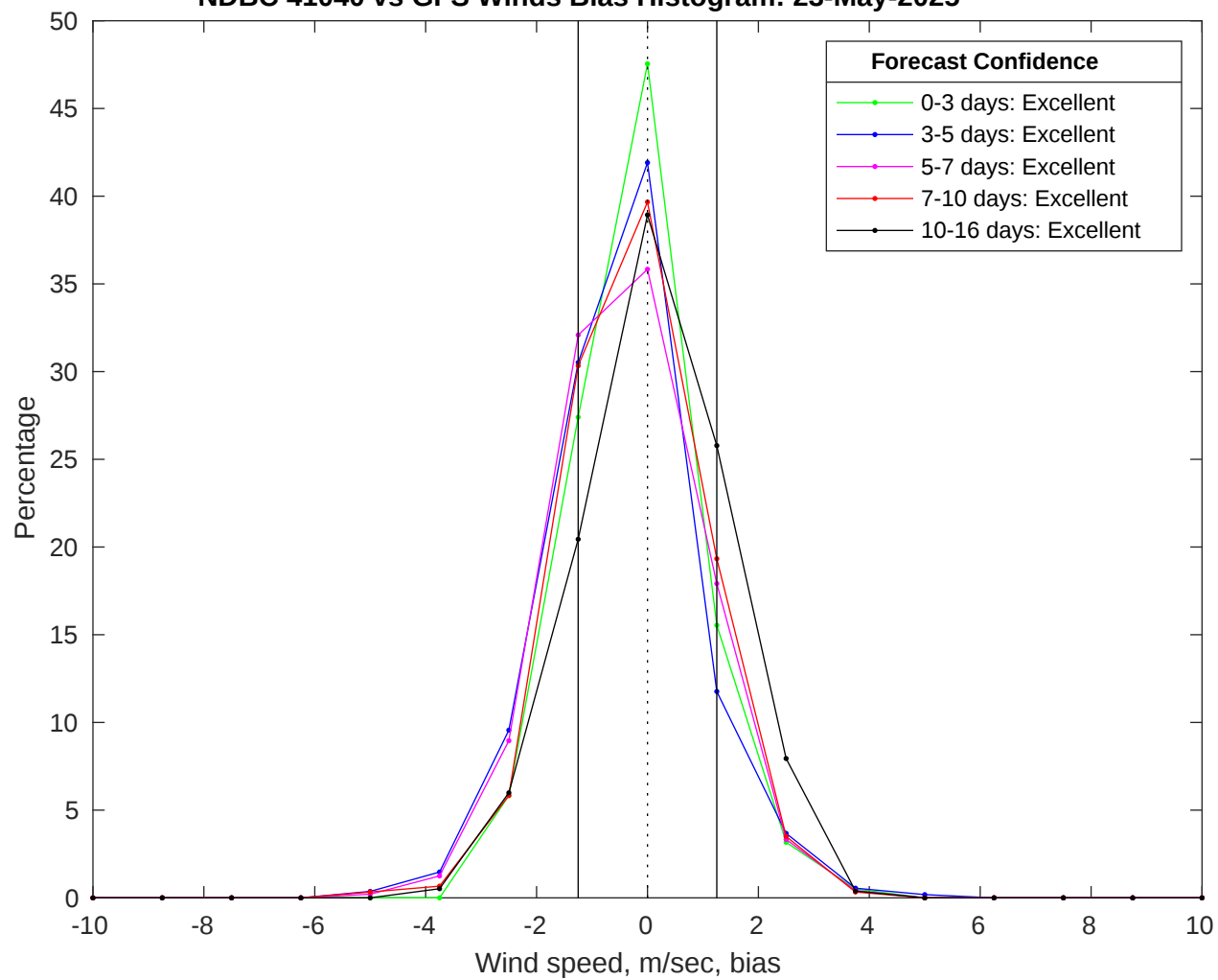
NDBC 41040 vs GFS Winds Bias Histogram: 23-May-2025
