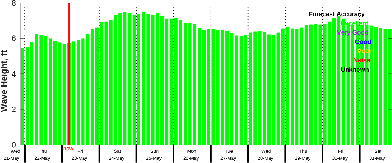
CMEMS Wave Forecast for NDBC 41040 from 21-May-2025 21:00:00 to 31-May-2025 21:00:00
