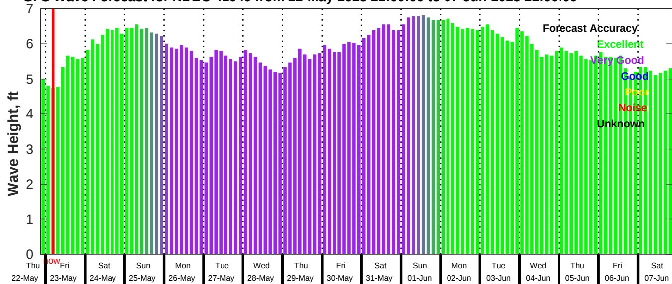
GFS Wave Forecast for NDBC 41040 from 22-May-2025 21:00:00 to 07-Jun-2025 21:00:00
