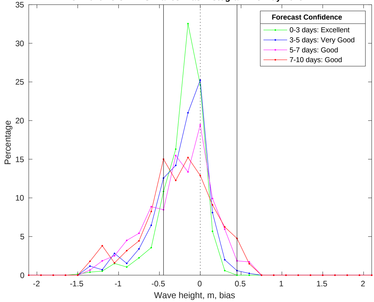
NDBC 42019 vs CMEMS Waves Bias Histogram: 23-May-2025
