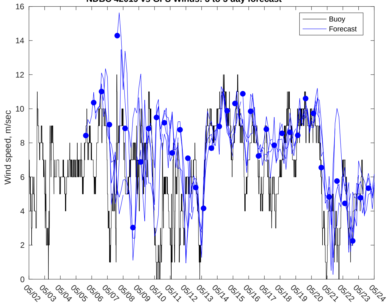
NDBC 42019 vs GFS Winds: 3 to 5 day forecast
