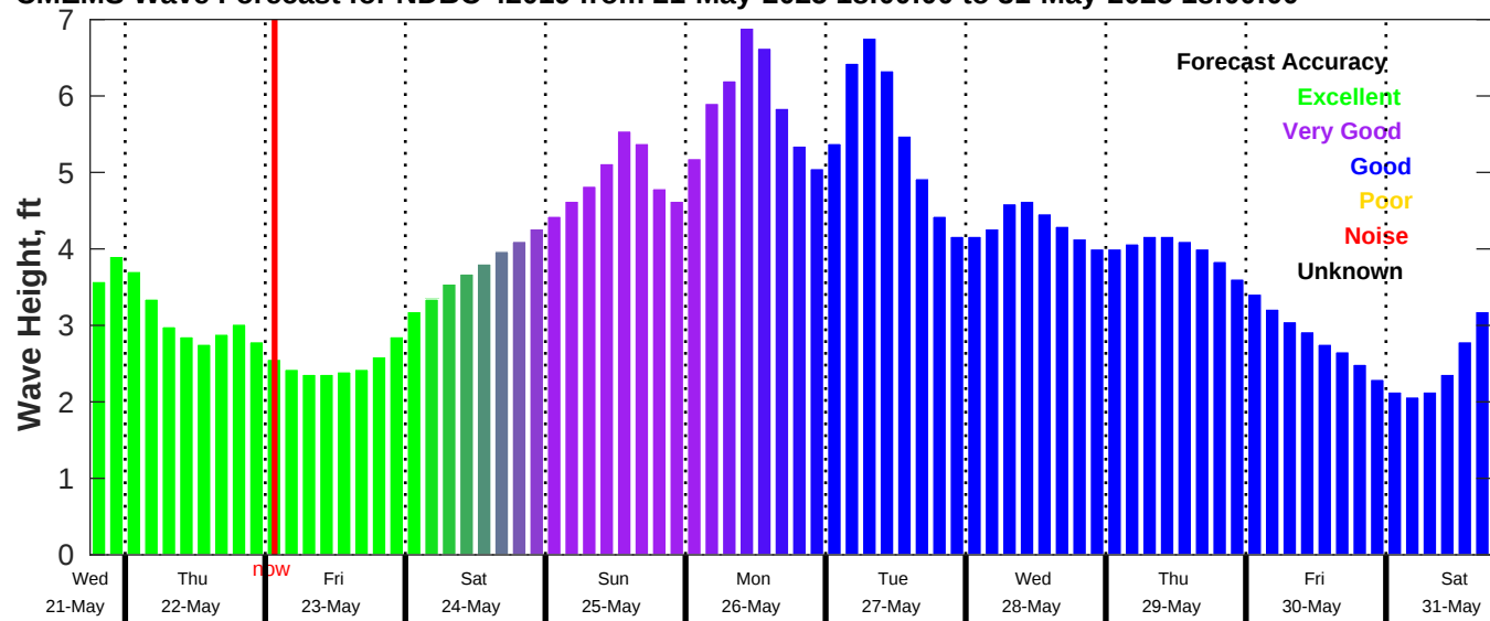
CMEMS Wave Forecast for NDBC 42019 from 21-May-2025 18:00:00 to 31-May-2025 18:00:00
