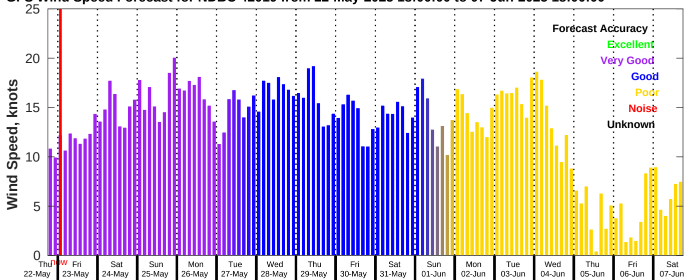
GFS Wind Speed Forecast for NDBC 42019 from 22-May-2025 18:00:00 to 07-Jun-2025 18:00:00
