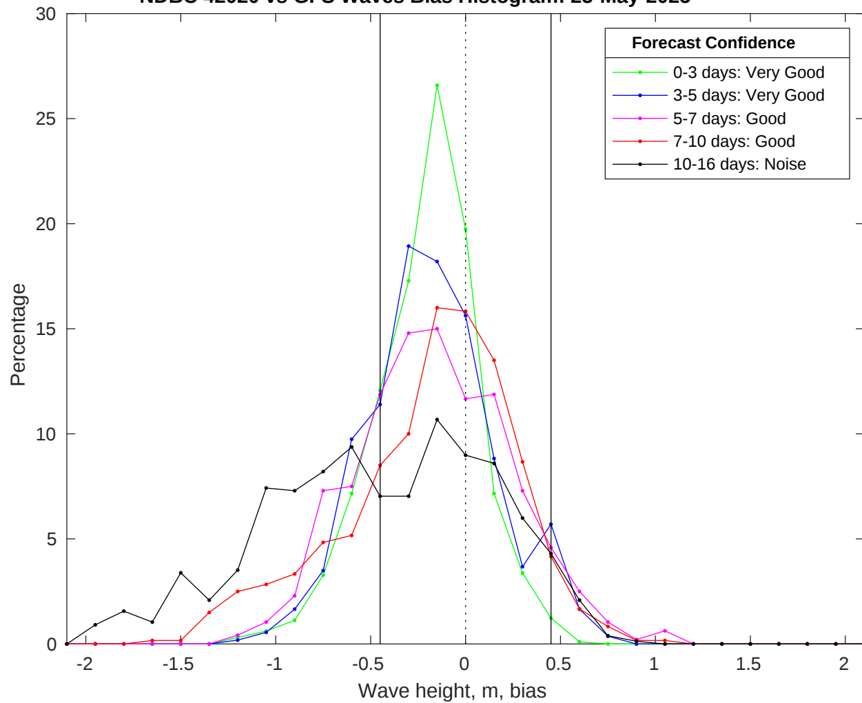
NDBC 42020 vs GFS Waves Bias Histogram: 23-May-2025
