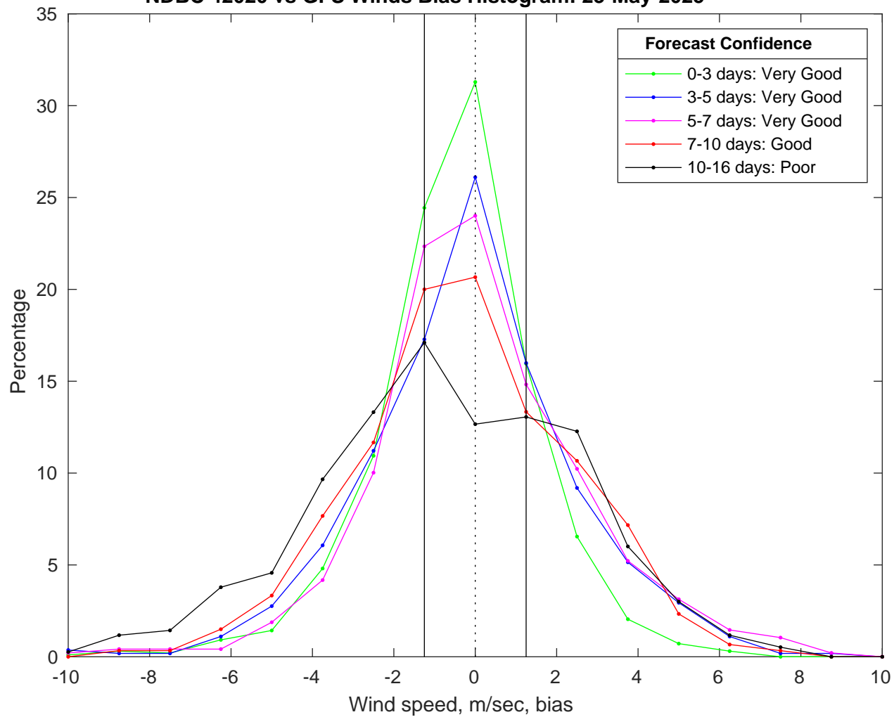
NDBC 42020 vs GFS Winds Bias Histogram: 23-May-2025
