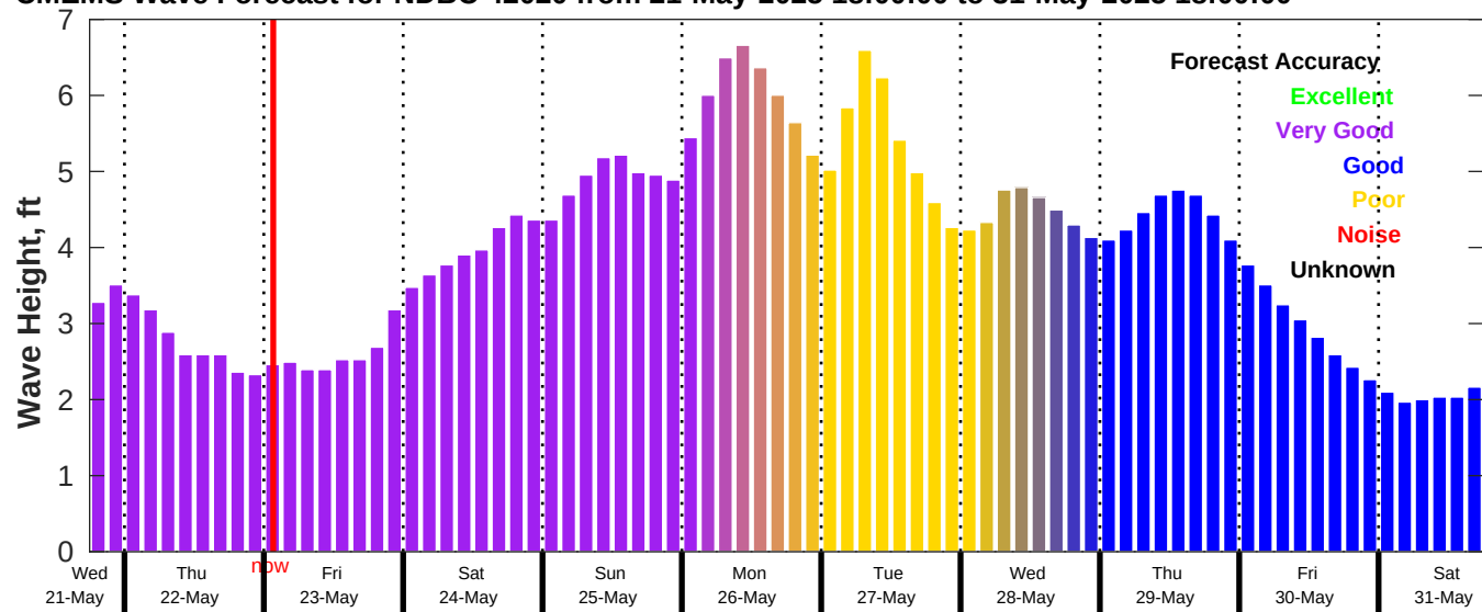
CMEMS Wave Forecast for NDBC 42020 from 21-May-2025 18:00:00 to 31-May-2025 18:00:00
