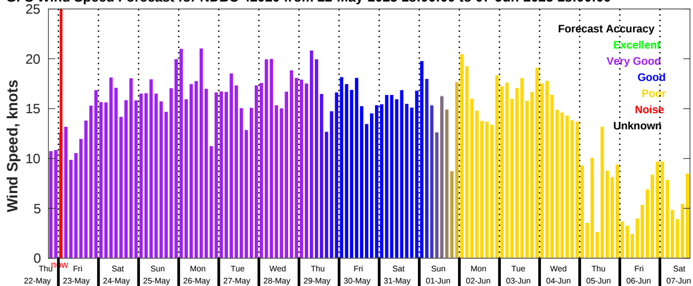
GFS Wind Speed Forecast for NDBC 42020 from 22-May-2025 18:00:00 to 07-Jun-2025 18:00:00
