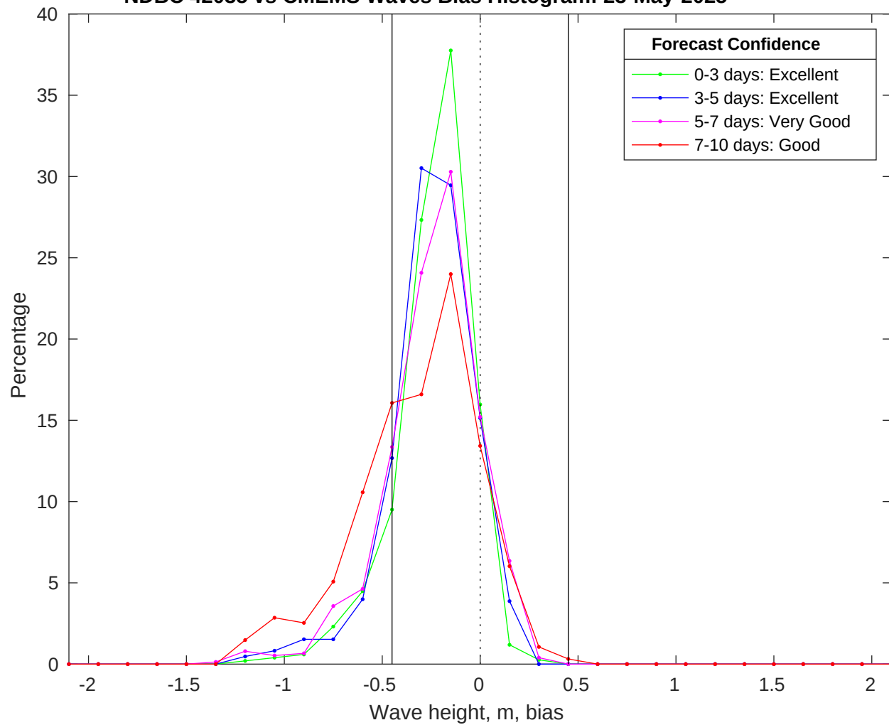
NDBC 42035 vs CMEMS Waves Bias Histogram: 23-May-2025
