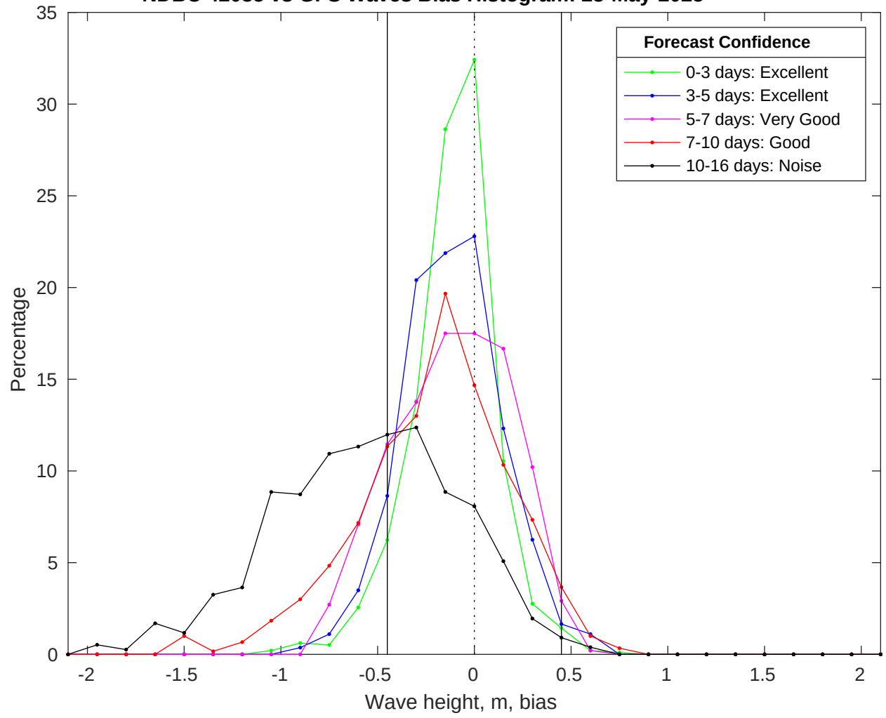
NDBC 42035 vs GFS Waves Bias Histogram: 23-May-2025
