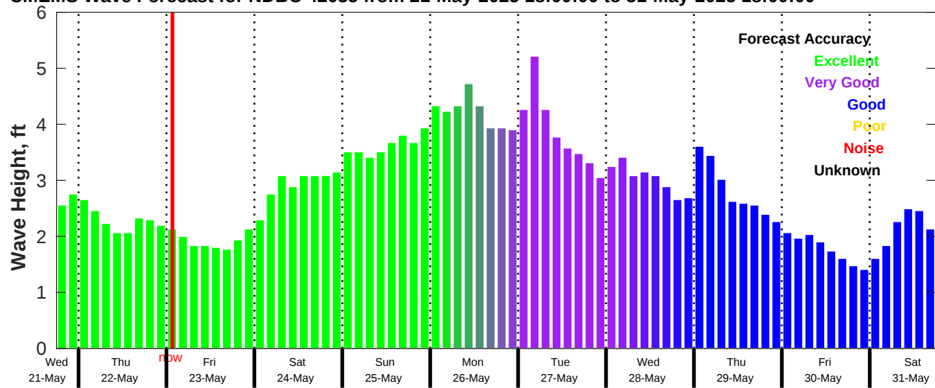
CMEMS Wave Forecast for NDBC 42035 from 21-May-2025 18:00:00 to 31-May-2025 18:00:00
