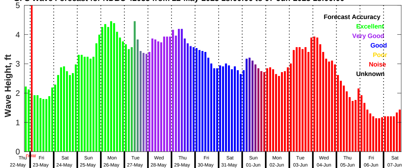
GFS Wave Forecast for NDBC 42035 from 22-May-2025 18:00:00 to 07-Jun-2025 18:00:00
