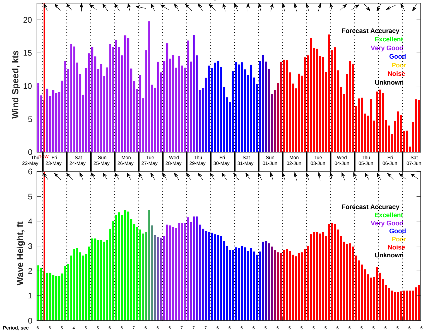
Wind & Wave Forecast for NDBC 42035 from 22-May-2025 18:00:00 to 07-Jun-2025 18:00:00
