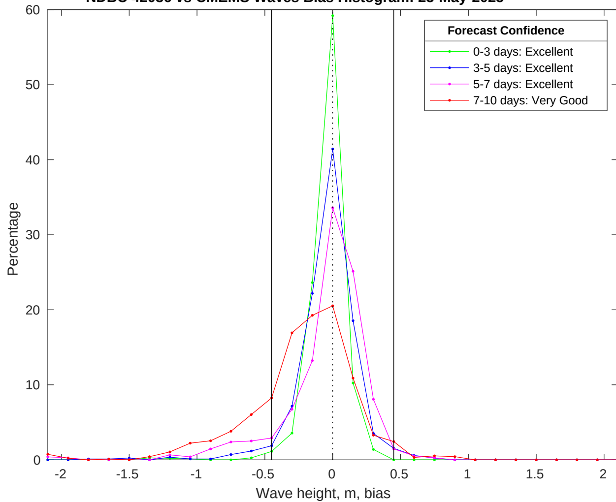
NDBC 42036 vs CMEMS Waves Bias Histogram: 23-May-2025
