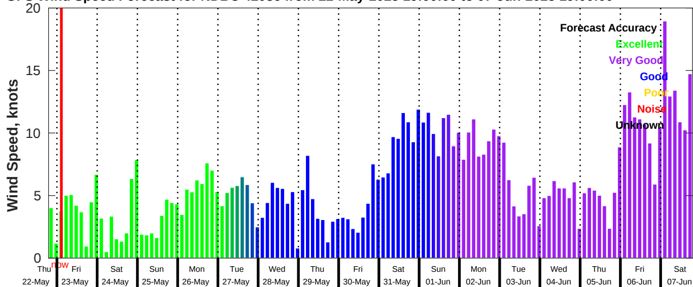
GFS Wind Speed Forecast for NDBC 42036 from 22-May-2025 19:00:00 to 07-Jun-2025 19:00:00
