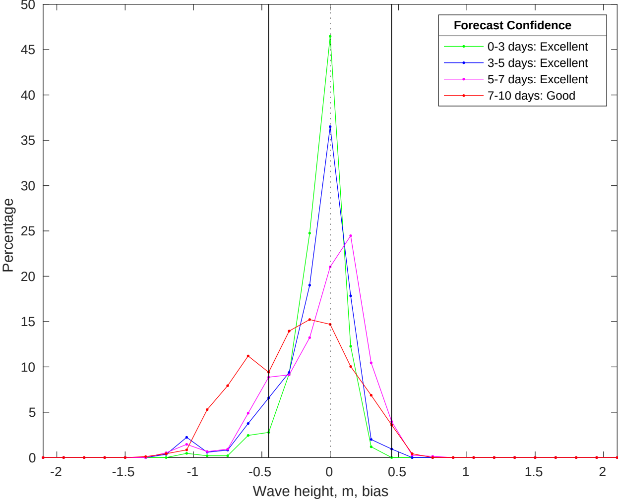
NDBC 42040 vs CMEMS Waves Bias Histogram: 23-May-2025
