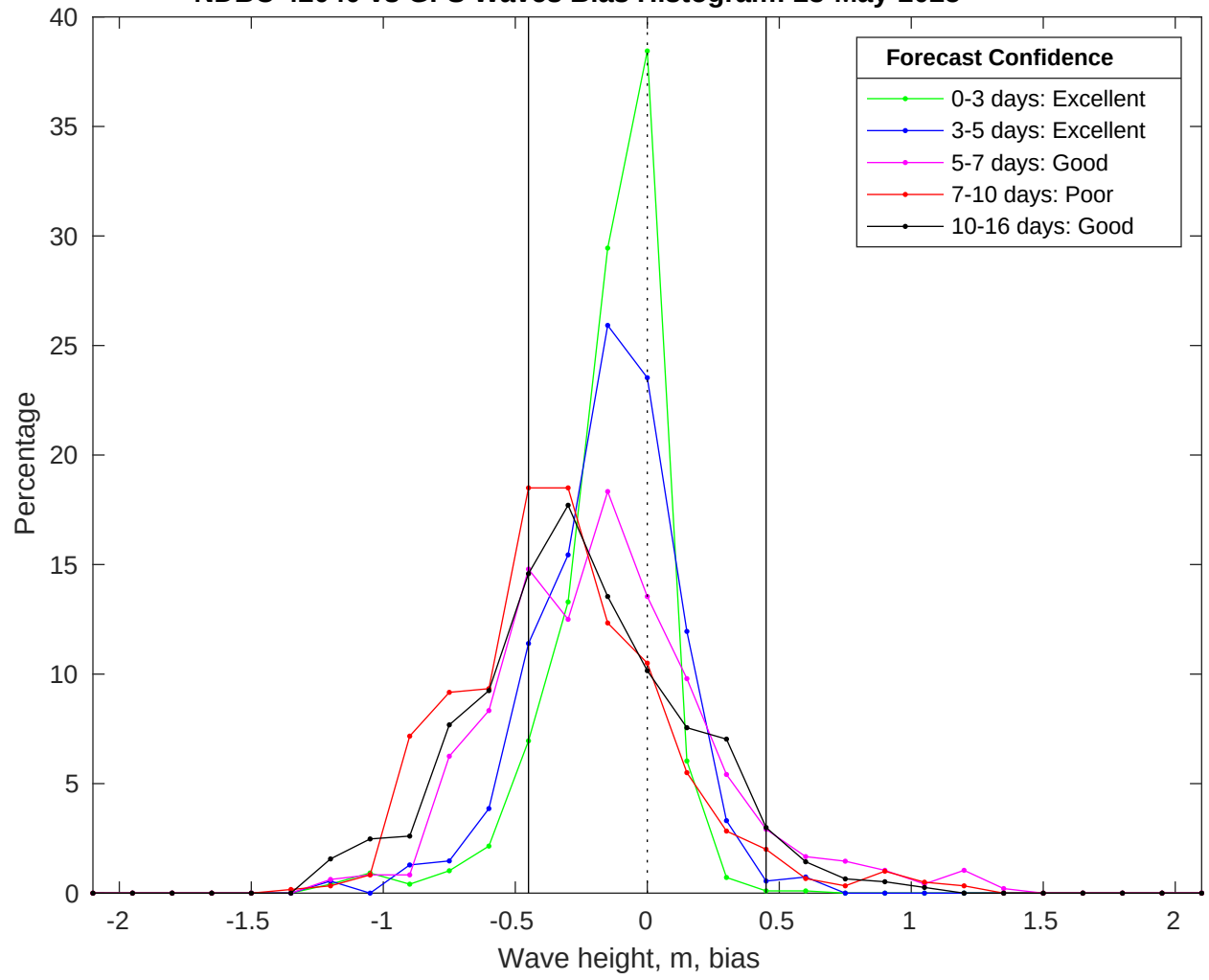
NDBC 42040 vs GFS Waves Bias Histogram: 23-May-2025
